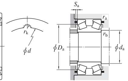
Bore key way
